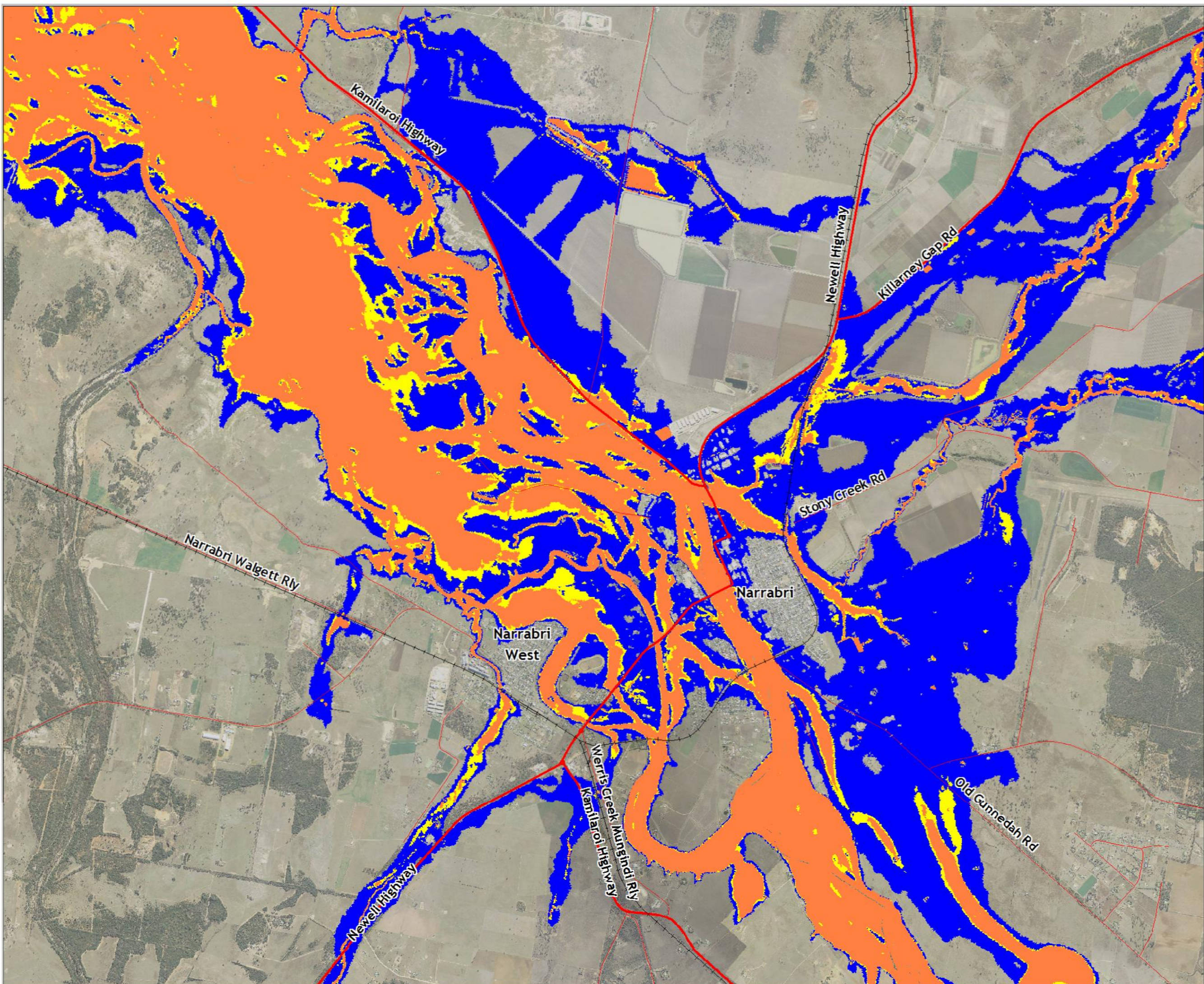
NARRABRI FLOOD STUDY Figure C.3: Preliminary Hydraulic Hazards 5% AEP Event
