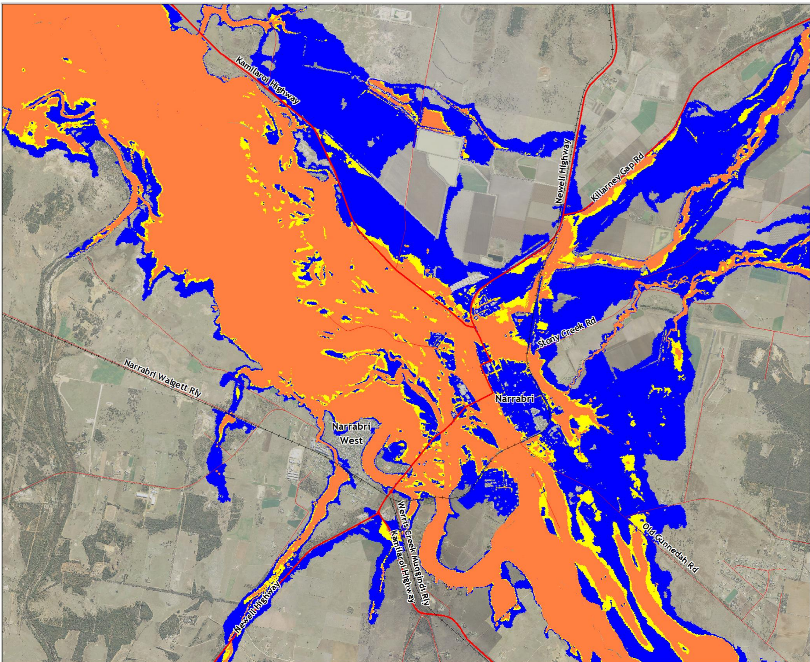
NARRABRI FLOOD STUDY Figure C.4: Preliminary Hydraulic Hazards 2% AEP Event
