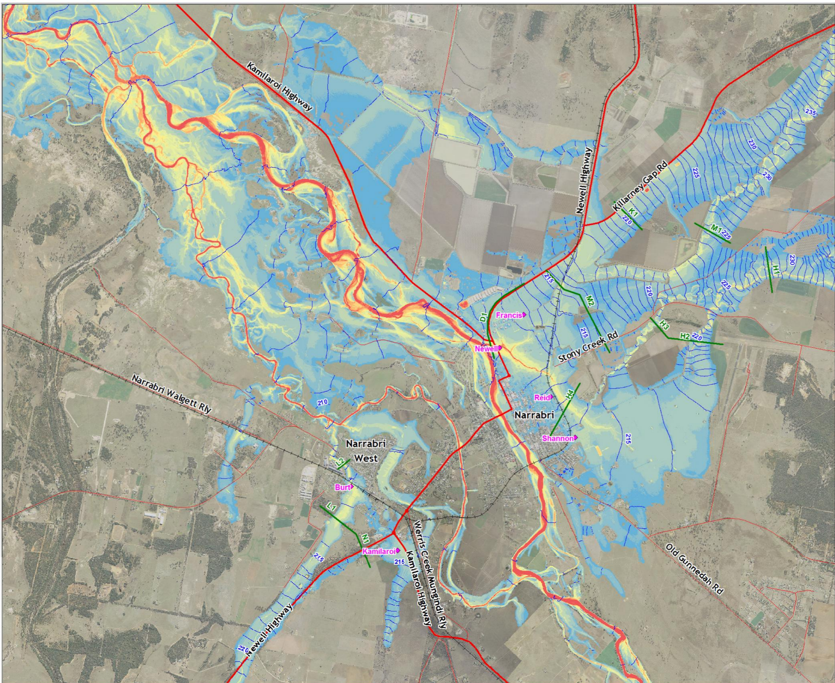
NARRABRI FLOOD STUDY Figure B.10: Predicted Flood Extent, Levels and Depth Local 1% AEP Event
