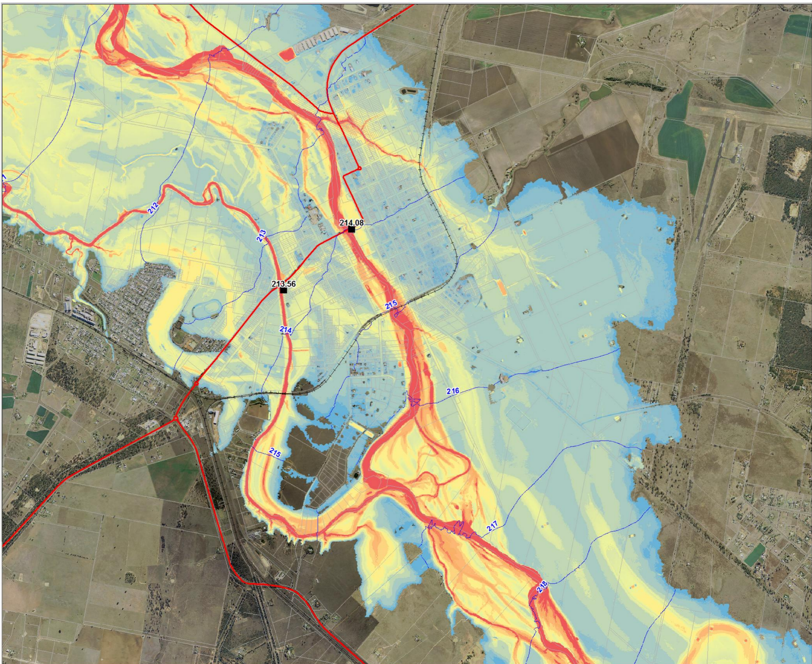
Figure B.9: Predicted Flood Extent, Level and Depth Regional 1% AEP Event
