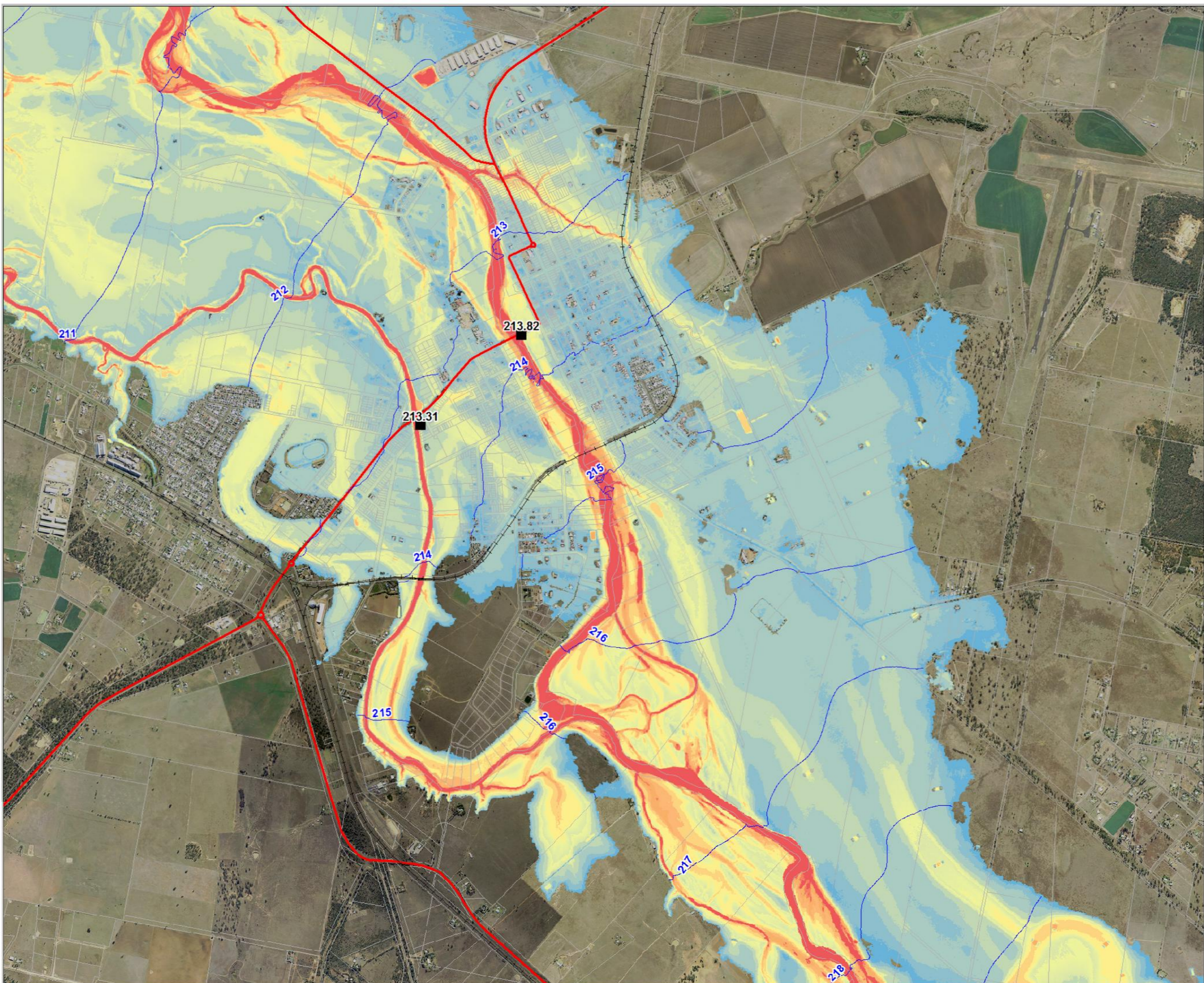
NARRABRI FLOOD STUDY Figure B.7: Predicted Flood Extent, Level and Depth Regional 2% AEP Event
