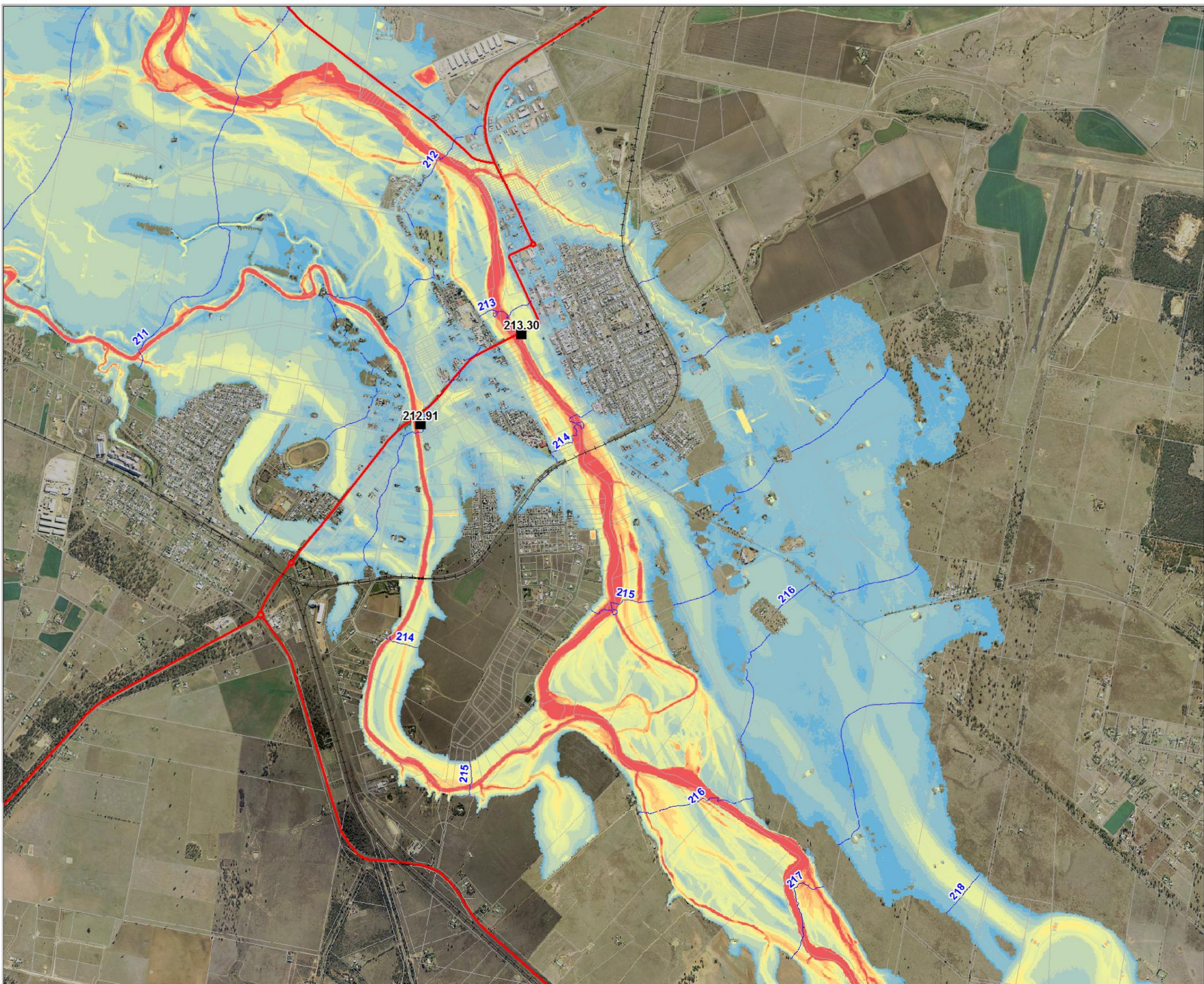
Figure B.5: Predicted Flood Extent, Level and Depth Regional 5% AEP Event
