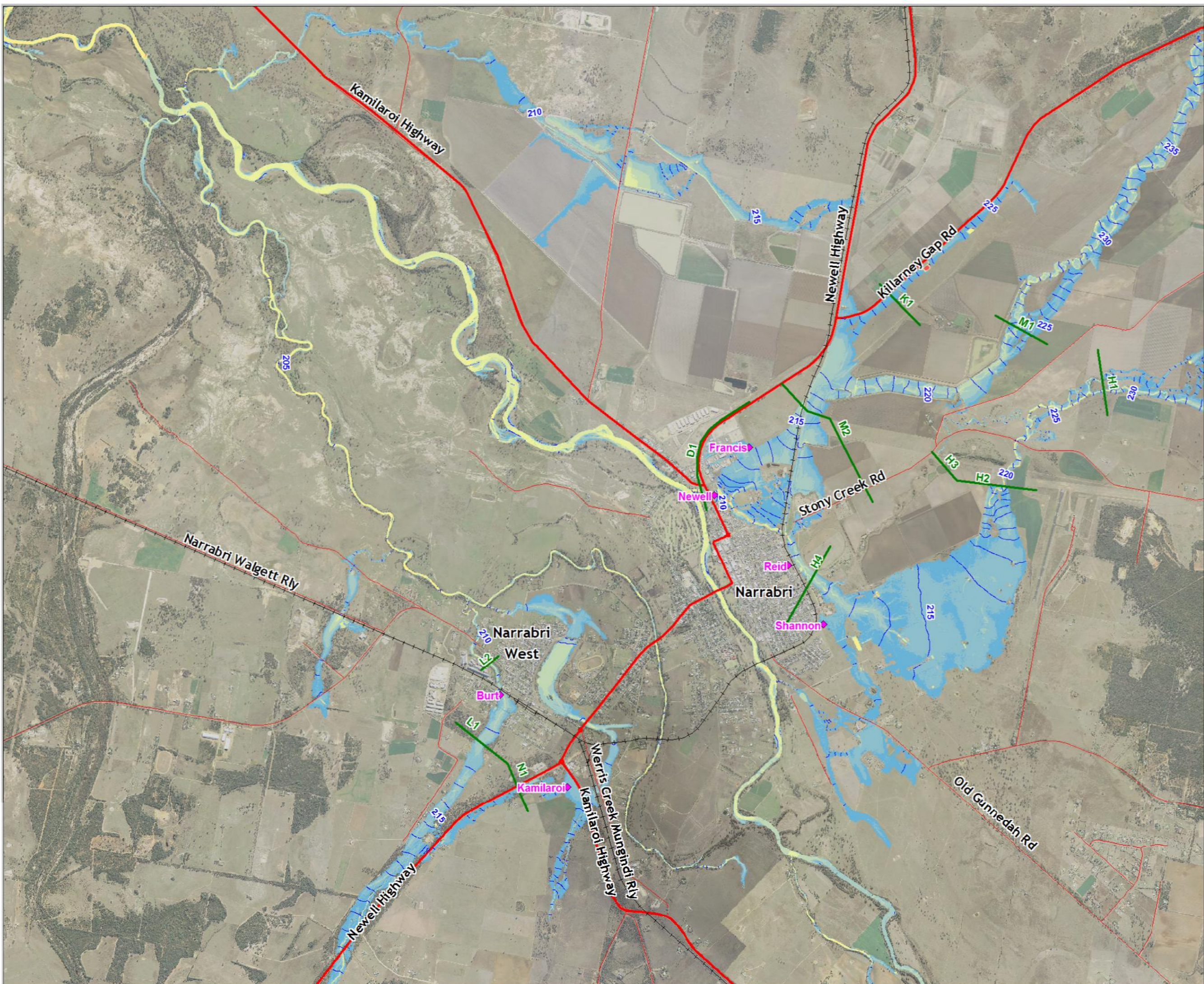
NARRABRI FLOOD STUDY Figure B.2: Predicted Flood Extent, Levels and Depth Local 20% AEP Event
